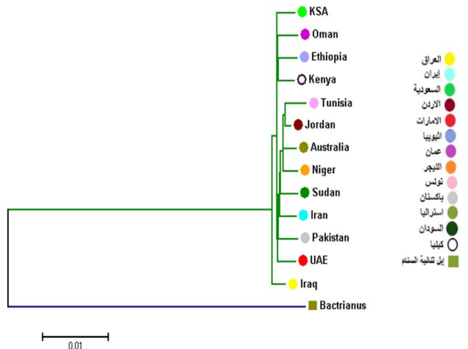
Figure 4: Neighbor-joining (NJ) tree of Iraq camels and reference sequences
