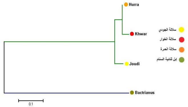
Figure 3: Neighbor-joining (NJ) tree of the tested Iraq camel breed Joudi, Khwar and Hurra.
