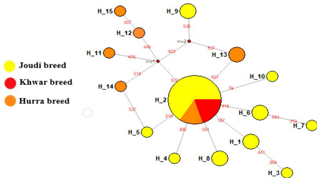
Figure 1: Median-joining networks constructed of the tested Iraq camel breed Joudi, Khwar, and Hurra.
